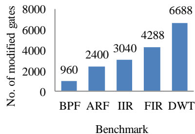
Fig. 13. # of gates affected (structural change) through proposed obfuscation.
