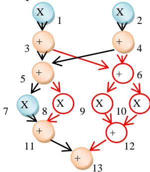
Fig.3. Proposed Redundant Operation Removal based obfuscation.
