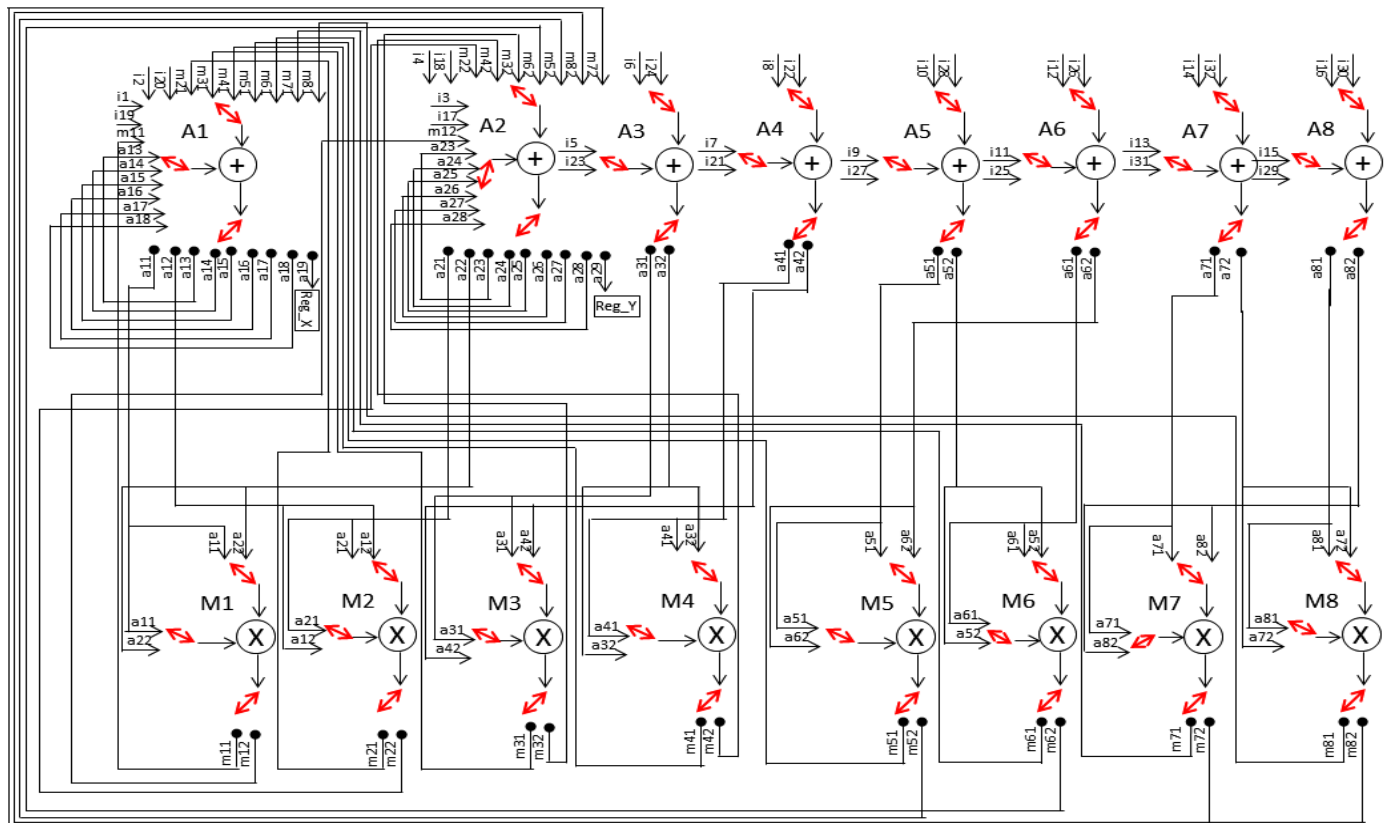
Fig. 11. Non-obfuscated DSP circuit of a FIR filter with normal fault security (no enhancement in fault security capability based on [31]).
