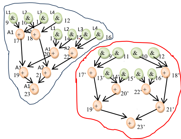
Fig.9. Proposed Obfuscated DMR design of a FIR filter
